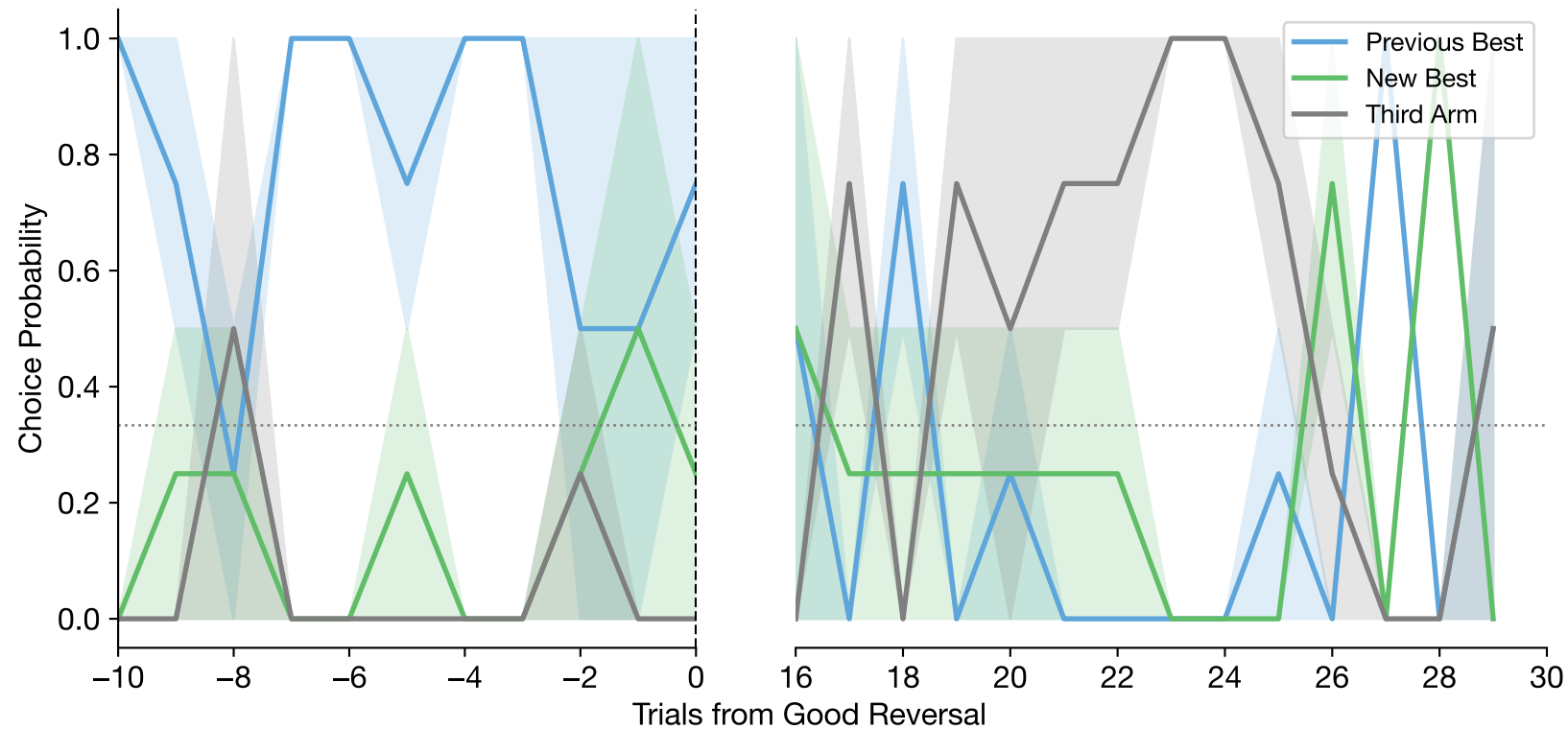
Good Reversal-Aligned Choices (mean \pm se across subjects | n=2 subjects, n=3 reversals) (Skipping first 15 trials post-reversal)
